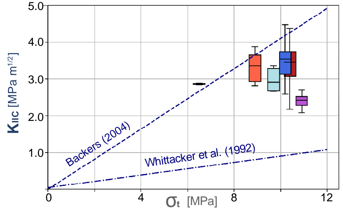
Fracture toughness mode II
