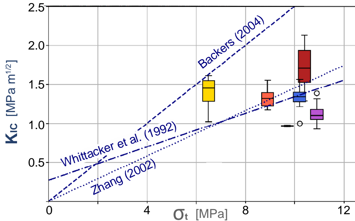
Fracture toughness mode I
